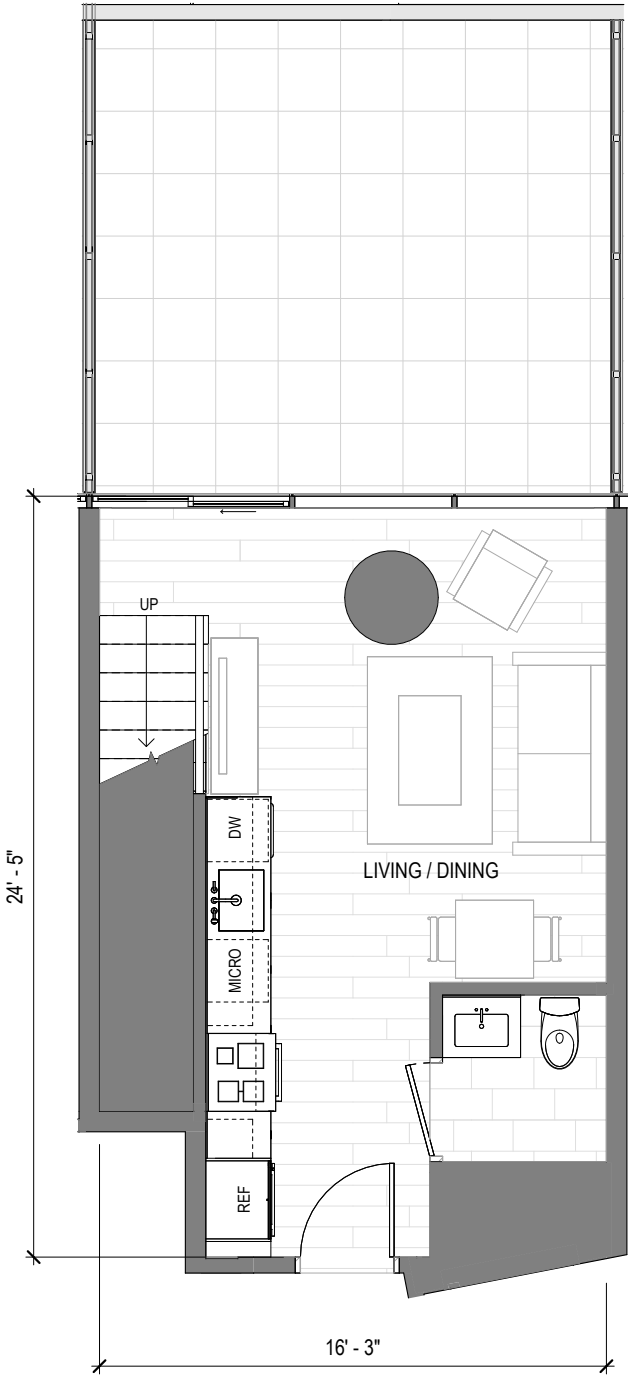
FIRST FLOOR
